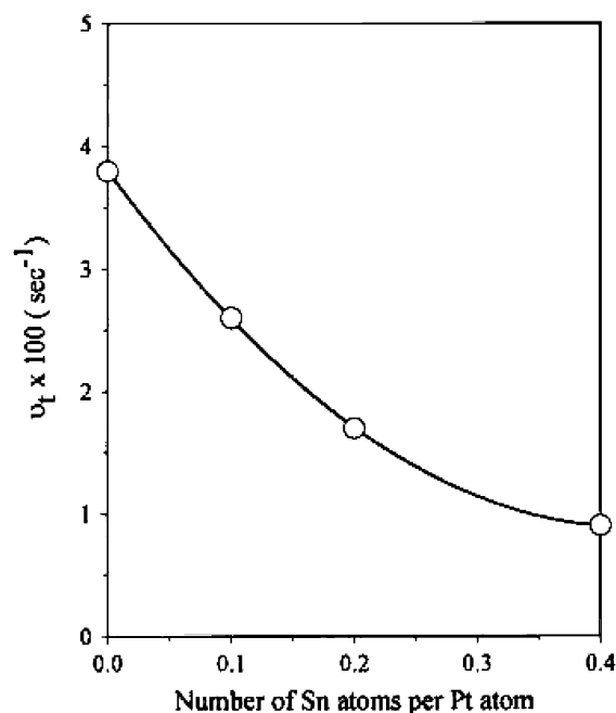
Figure 5. The catalytic activity of n -hexane aromatization over the PtSn/KL catalysts plotted against the atomic ratio of Sn/Pt. The reaction was performed at 671 \pm 1 K with H_2/C_6H_{14}=6 . v_t was based on the total amount of Pt.
